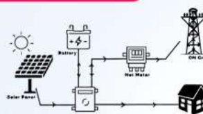
HYBRID SYSTEM
